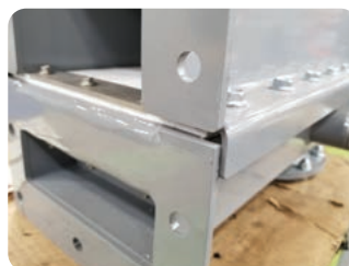
Rain ledge prevents precipitation from leaking into the conveyor
